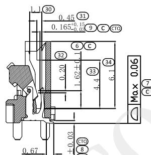
SECTION A-A ACT OPEN
