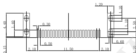
PCB PATTERN LAYOUT
