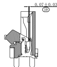
SECTION A-A ACT CLOSE
