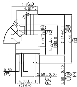
SECTION A-A ACT CLOSE
